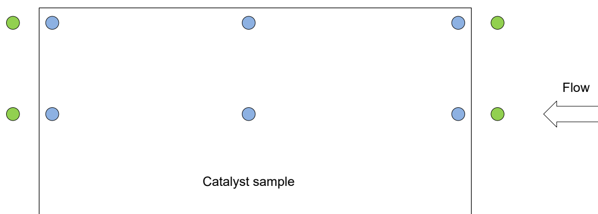
Figure 2 Thermocouple positions
