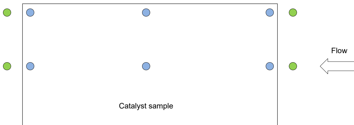
Figure 2 Thermocouple positions
